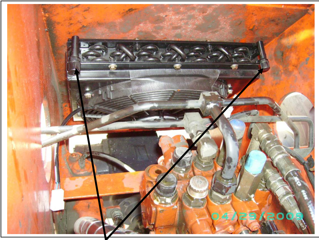
R520 shown. Fittings go toward the bottom on the R420.
